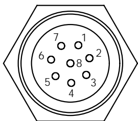
MIC/LINE IN LEFT CONNECTOR
